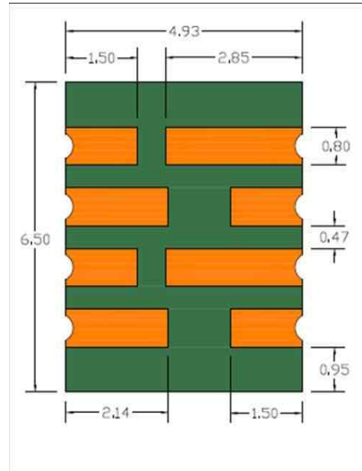
Fig.6 Recommended PCB metal pattern for HT-01S.
