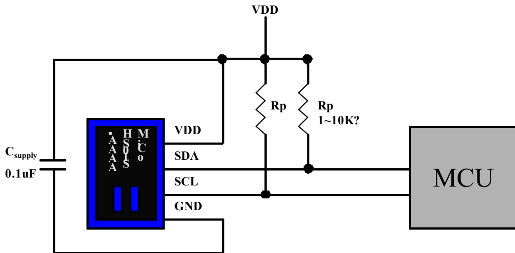
Fig.10 HT-01S I 2 C Interface
