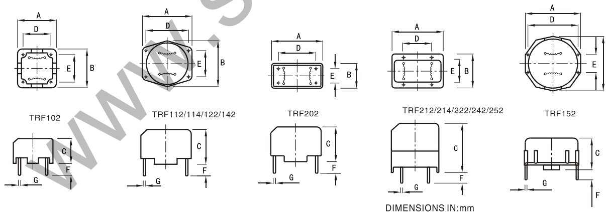
DIMENSIONS IN:mm
