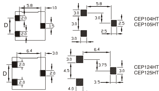
LAND PATTERN
