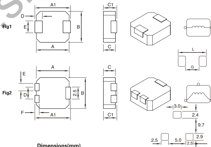
Dimensions(mm)
