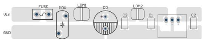
Fig.7 Recommended EMC circuit-PCB layout
