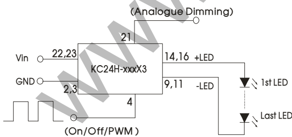
Fig. 2 Application circuits in series
