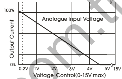
Fig. 10 Analogue Input voltage and output current
