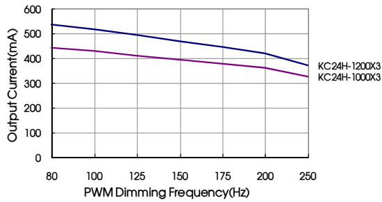
Fig. 7 PWM dimming frequency and output current (D=50%)
