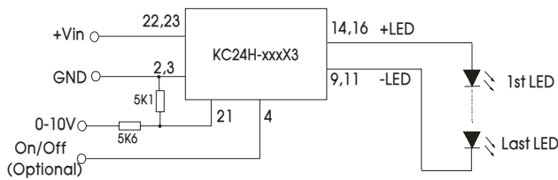
Fig. 9 Analogue dimming circuit
