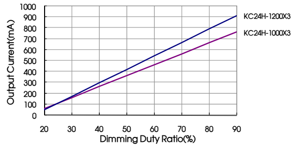
Fig. 8 Dimming duty ratio and output current (f=200Hz)
