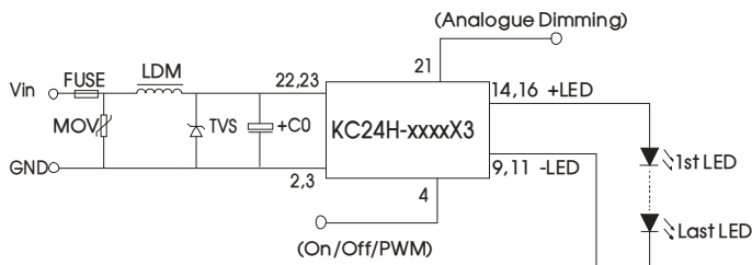
Fig.5 Recommended EMC circuit
