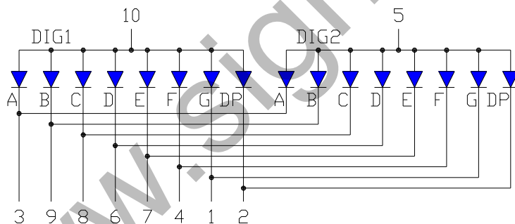
OPS-D3910LB-GW (Common Anode)
