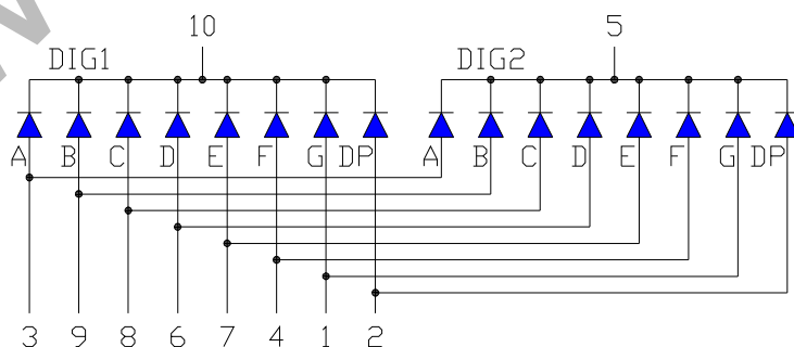
OPS-D3911LB-GW (Common Cathode)
