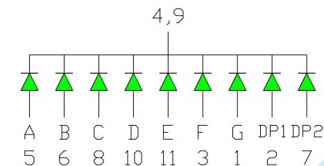
12 PIN No Connect OPS-S2811PG-GW (Common Cathode)
