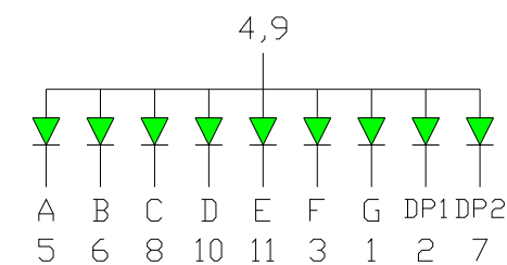
12 PIN No Connect OPS-S2812PG-GW (Common Anode)
