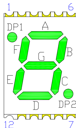
12 PIN No Connect OPS-S2812PG-GW (Common Anode)
