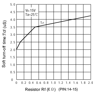
The reference curve of soft turn-off time & R f
