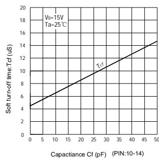
The reference curve of soft turn-off time & C f
