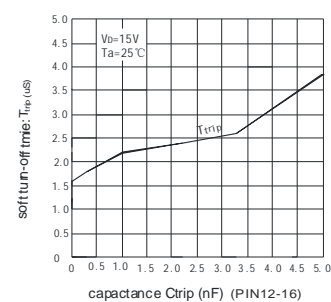
The reference curve of Controlled time detect short circuit & C trip
