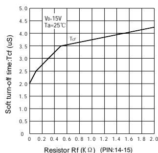
The reference curve of soft turn-off time & Rf
