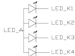
DETAIL A LED CIRCUIT DIAGRAM SCALE 40:1
