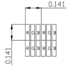
DETAIL A LED CIRCUIT DIAGRAM SCALE 40:1
