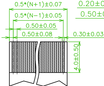
FPC/FFC T=0.30±0.03mm
