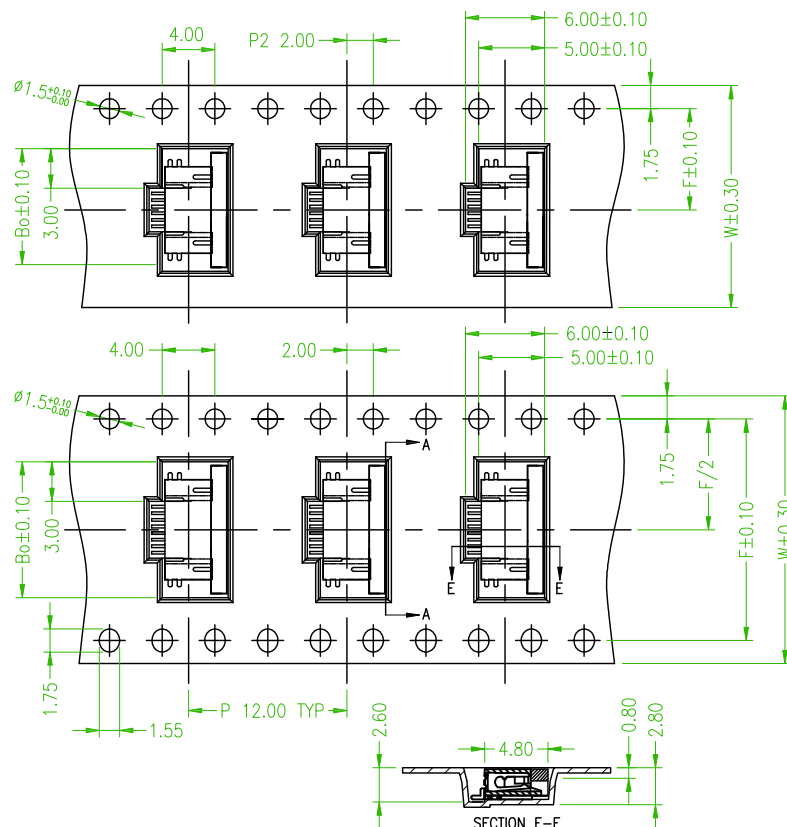
SECTION E-E
