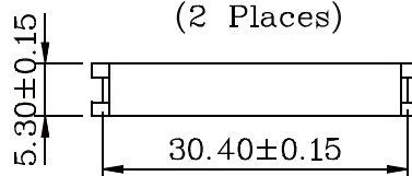
Termination Cover (2 Places)
