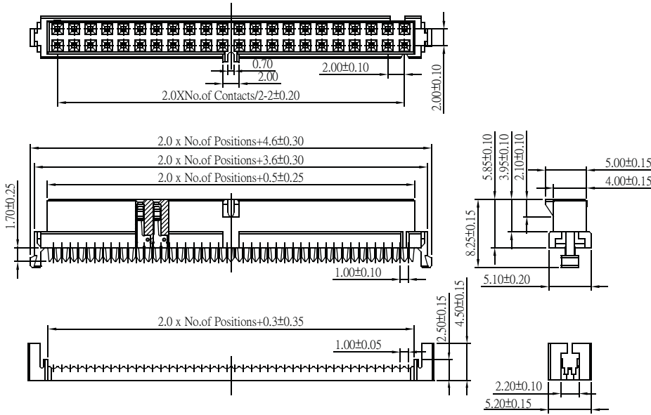
Part No.: IDC2A-XX-L
