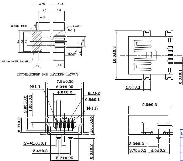
Part No.:MUSB-BS-5-U
