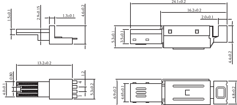
Part No.:MUSB-M4S-BB-L
