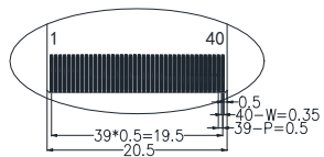
DETAIL A (4:1)
