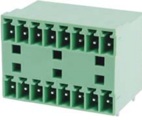
TB15ERH-3.5 TB15ERH-3.81 3.5mm 3.81mm / 22.7mm
