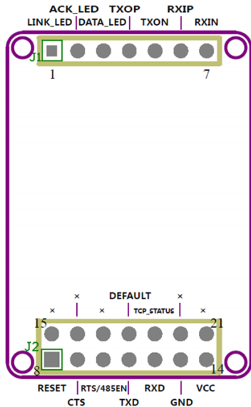
Figure 2-3 W7500S2E-S1 pinout
