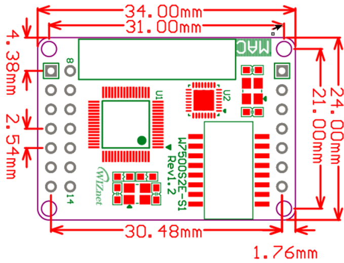
Figure 1-5 W7500S2E-S1 dimension - top view
