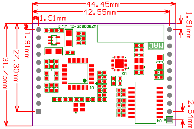
Figure 1-1 W7500S2E-Z1 dimension - top view
