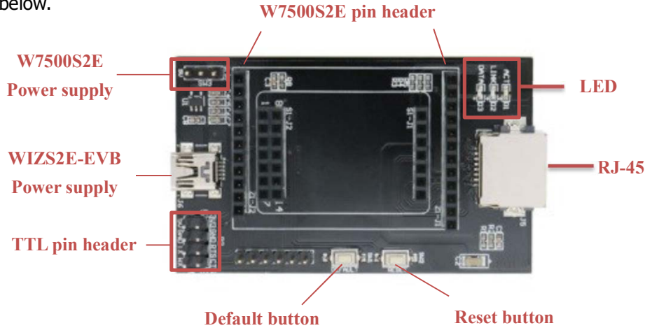
Figure 2-4 WIZS2E breakout board
