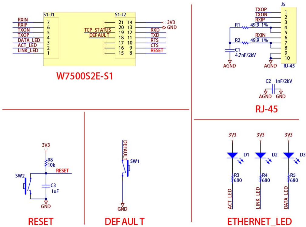
Figure 2-6 W7500S2E-S1 reference schematic
